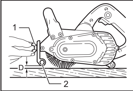
▶ 1. Wing nut 2. Front roller
