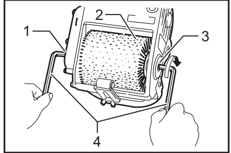
▶ 1. Spindle 2. Wheel 3. Output shaft 4. Hex wrench
